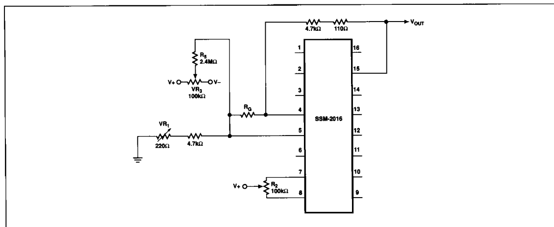
FIGURE 8: Trimming Circuit
