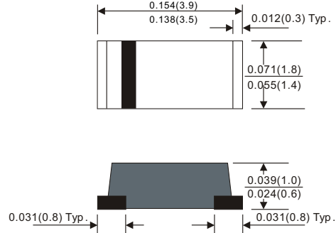
SOD-123
