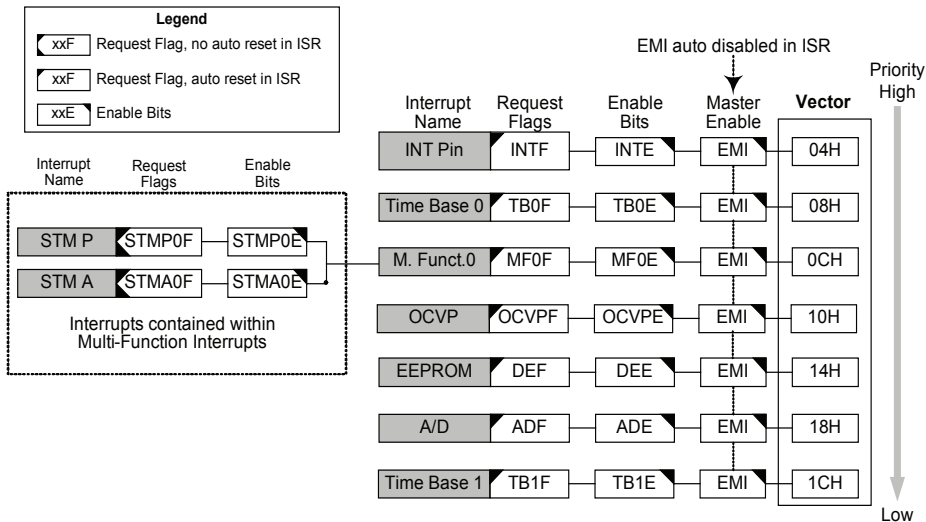
Interrupt Structure
