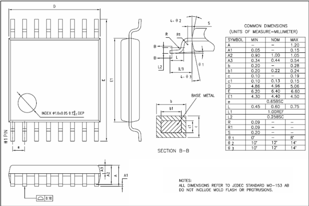
16 TSSOP(4.4mm) Pin Dimension (dimensions in millimeters)
