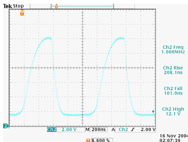
with RC filter
