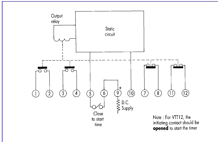
Figure 3: Typical connection diagram for dc VTT 11 relays
