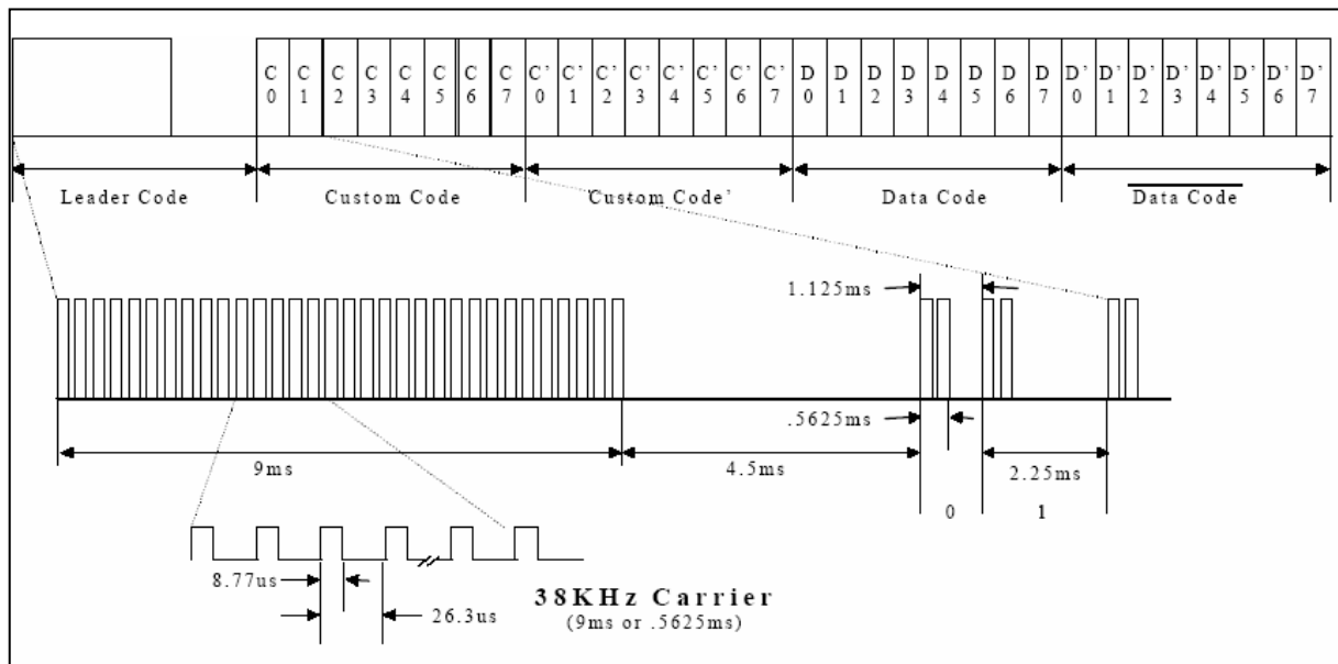
Figure 15-1.NEC CIR Frame Format
