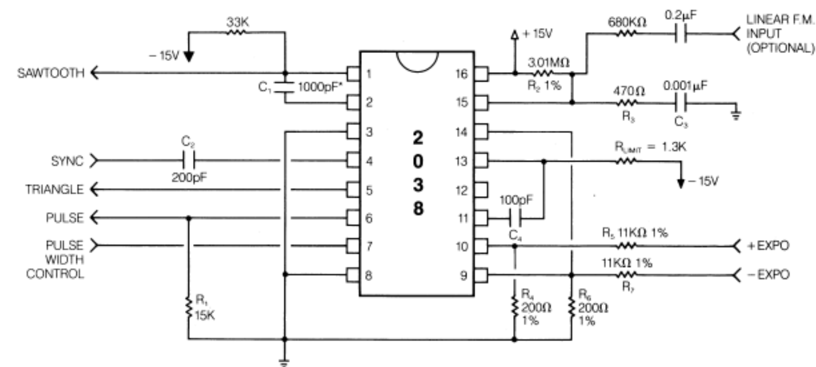
FIGURE 2. TYPICAL CONNECTION.
