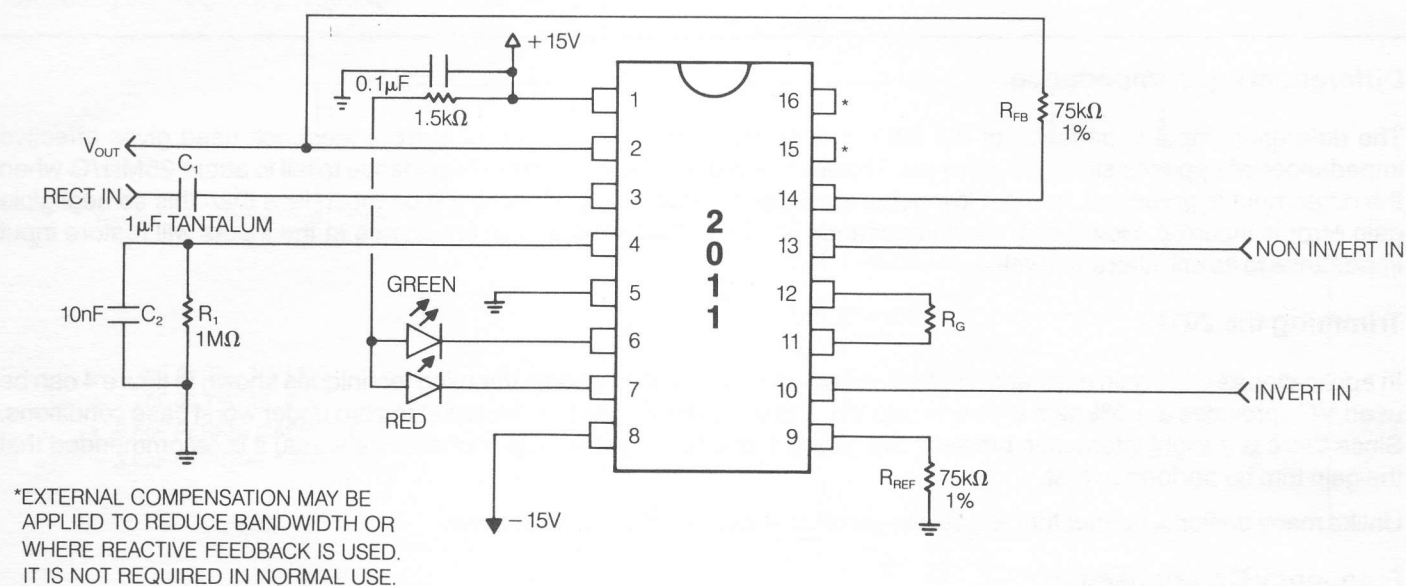
FIGURE 2. STANDARD CONFIGURATION. R_G = \frac{150k\Omega}{\text{REQUIRED GAIN}}
