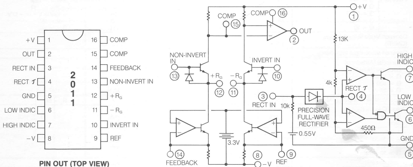
FIGURE 1. BLOCK DIAGRAM
