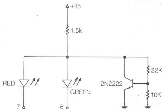
FIGURE 6. L.E.D. VOLTAGE CLAMP
