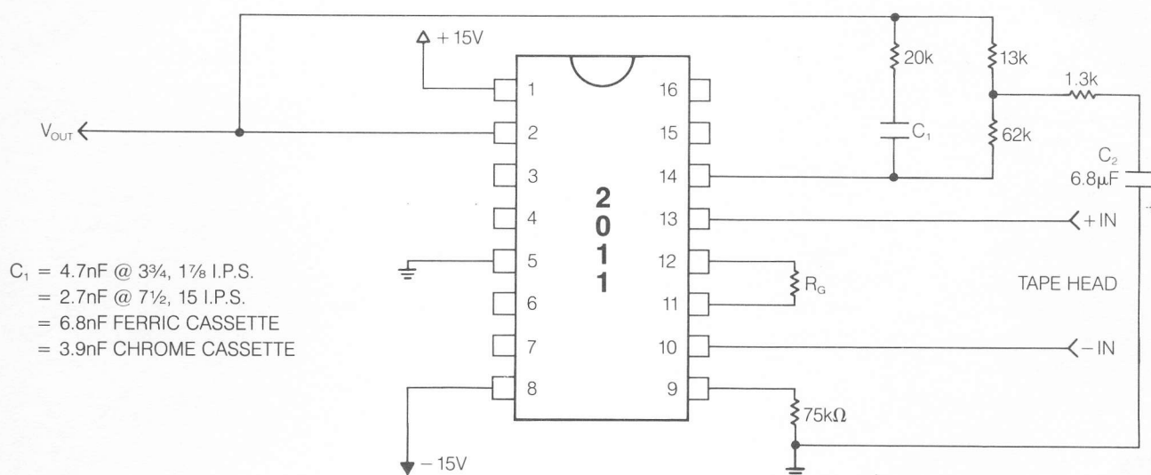
FIGURE 5. TAPE PLAYBACK PREAMPLIFIER
