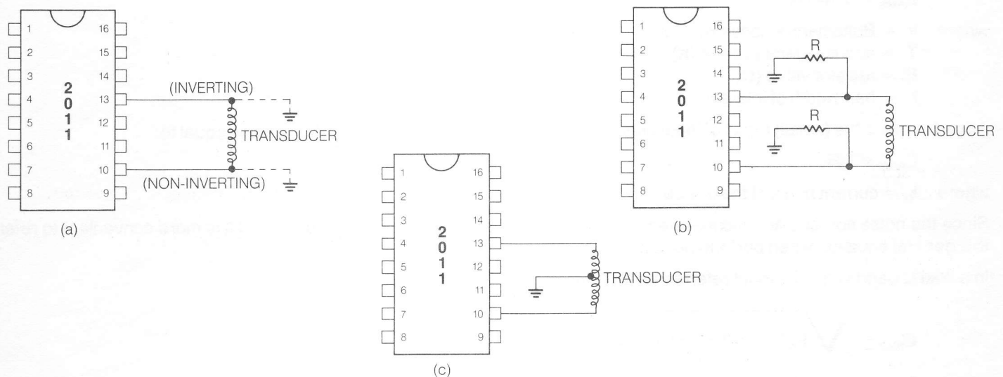
FIGURE 3. THREE WAYS OF INTERFACING TRANSDUCERS FOR HIGH NOISE IMMUNITY.
