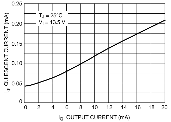
Figure 19. Quiescent Current vs. Output Current (Low Load)
