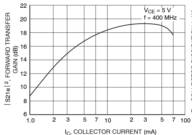
Figure 9. |S_{21e}|^2 – I_C
