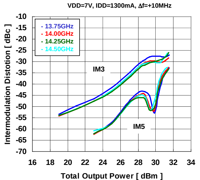
IMD vs TOTAL OUTPUT POWER
