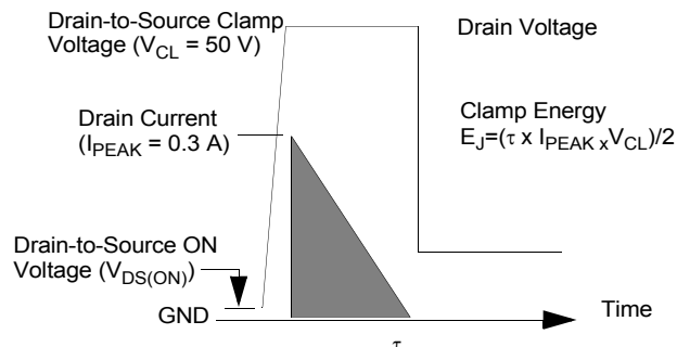
Figure 5. Output Voltage Clamping
