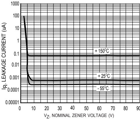
Figure 8 Typical Leakage Current
