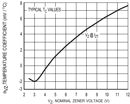
Figure 1 Temperature Coefficients (Temperature Range -55°C to +150°C)
