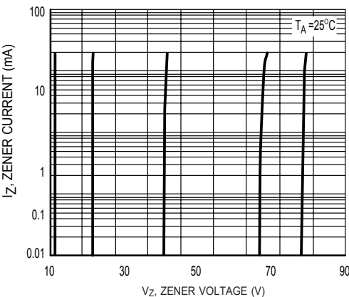
Figure 10 Zener Voltage vs. Zener Current (12 V to 43V)
