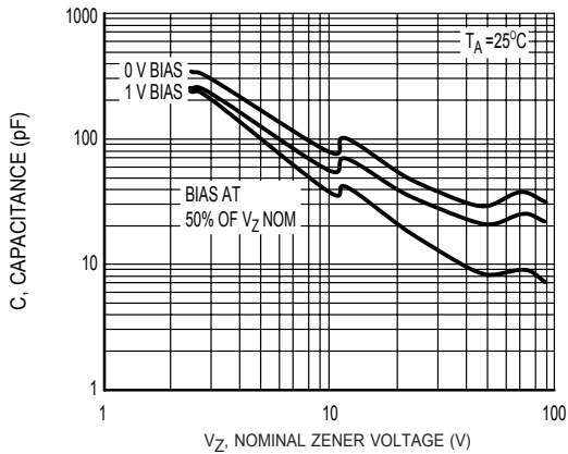
Figure 7 Typical Capacitance
