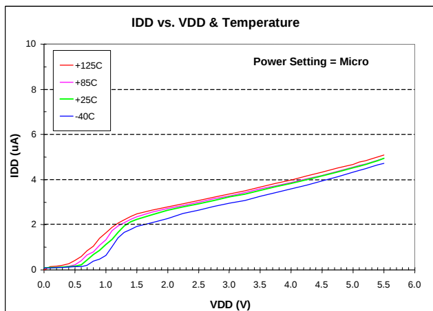
Figure 21 Supply Current (Micro Power)
