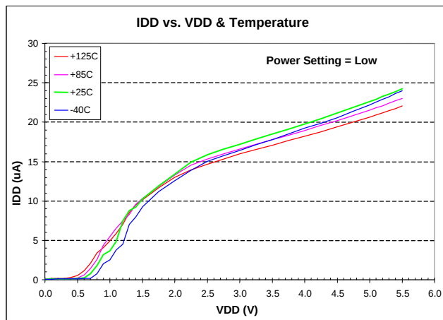
Figure 22 Supply Current (Low Power)
