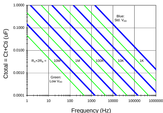
Figure 14 – Astable Frequency Chart (Std. Mode)
