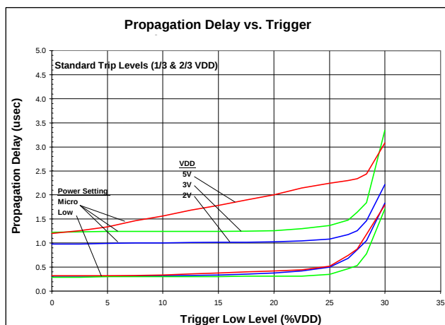
Figure 25 Propagation Delay (Standard V_{DD} )
