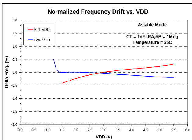
Figure 23 Frequency Drift vs. V_{DD}
