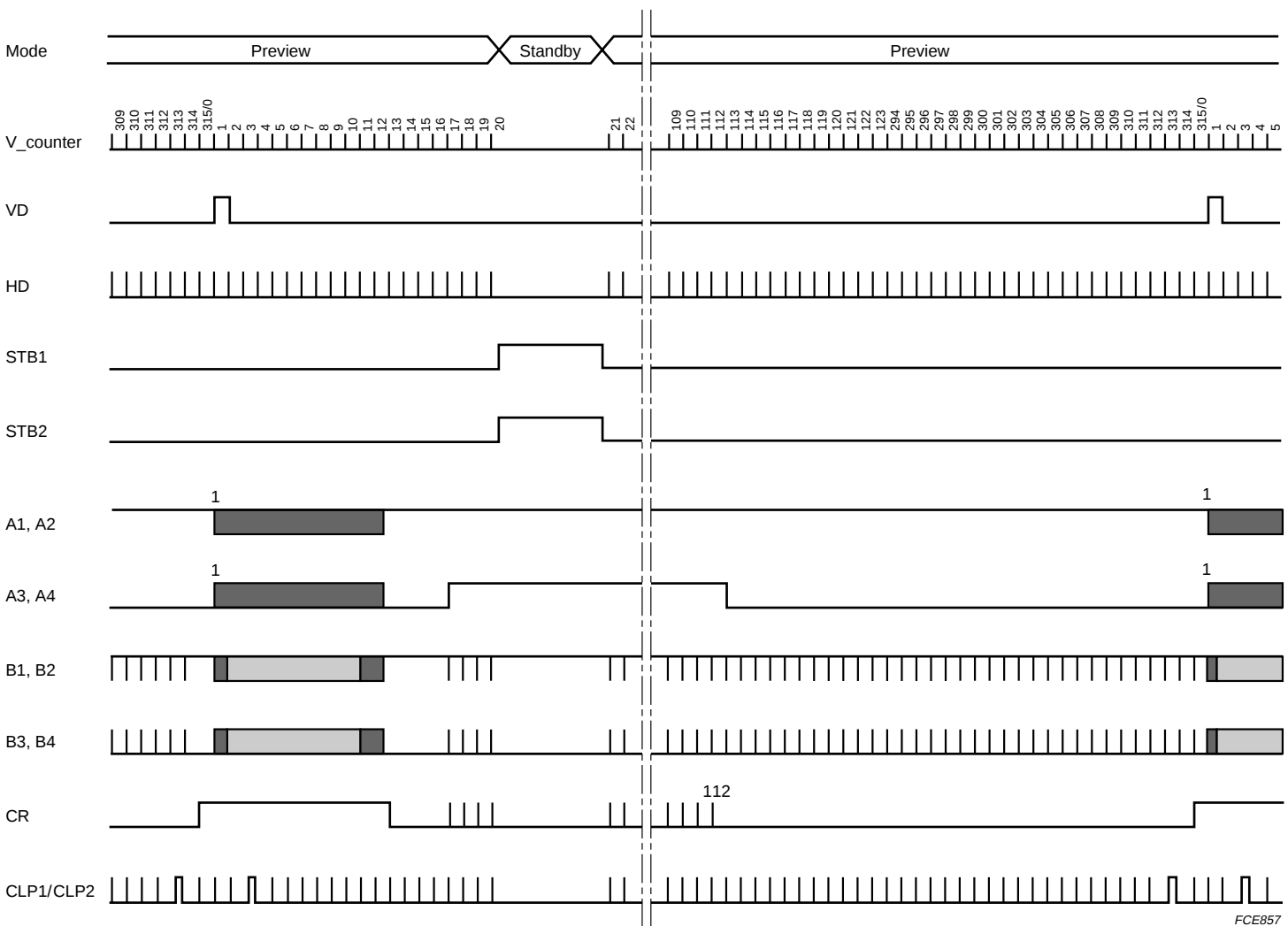
Fig.7 FT CCD V-driver timing in Preview mode with Standby mode 3.
