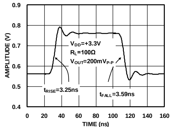
Figure12. Large-Signal Pulse Response Vs. Time(FHD Channel)
