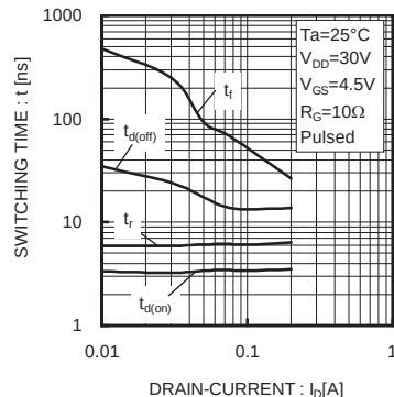
Fig.13 Switching Characteristics
