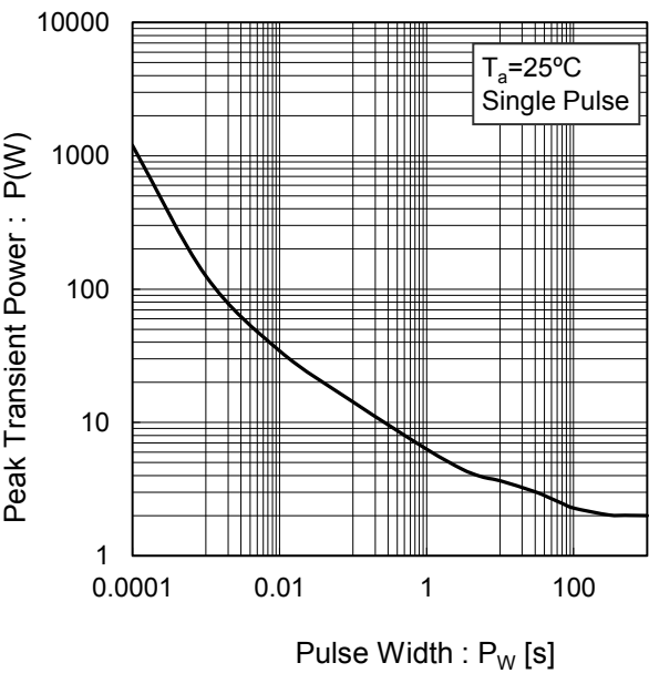
Fig.4 Single Pluse Maximum Power dissipation
