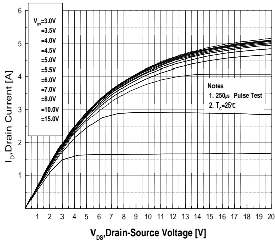
Fig.1 On-Region Characteristics
