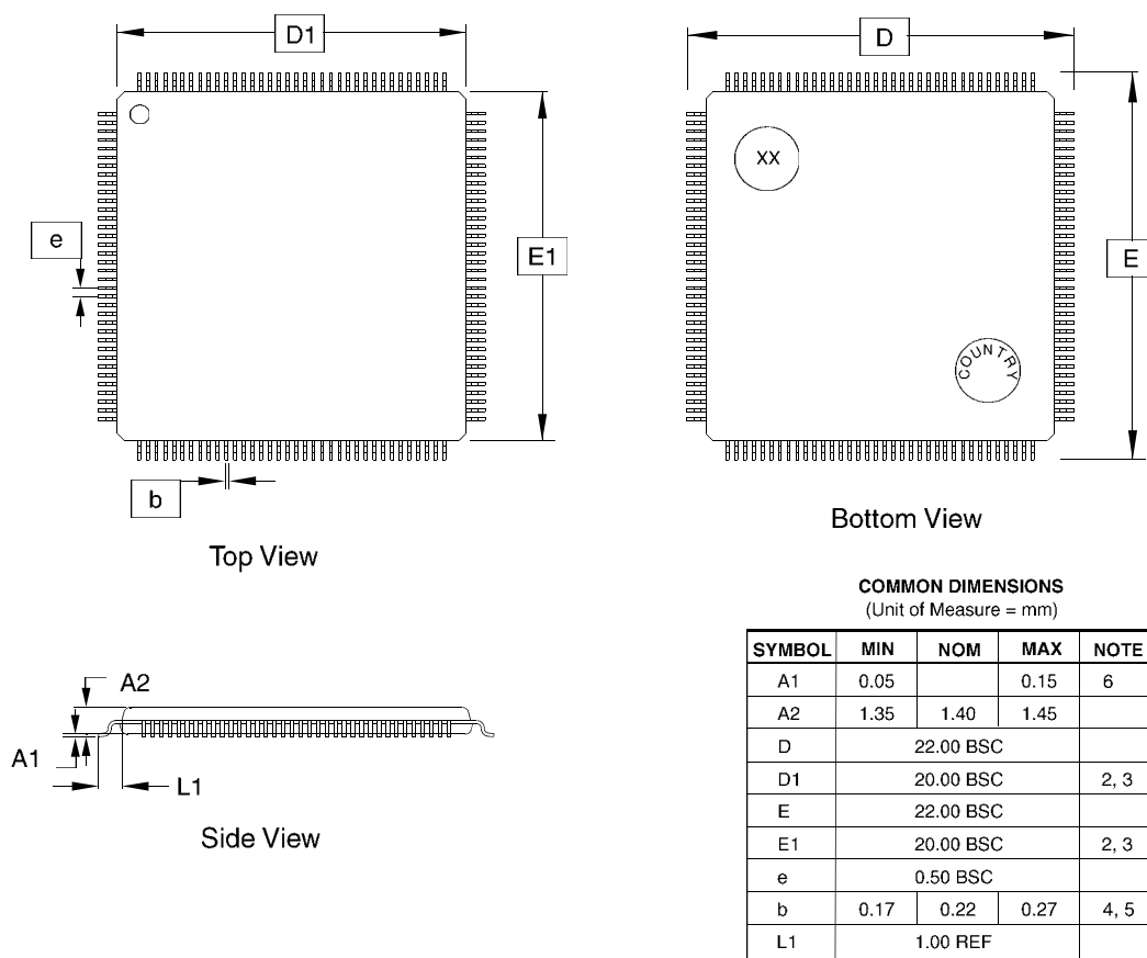
Figure 43-3. 144-lead LQFP Package Drawing
