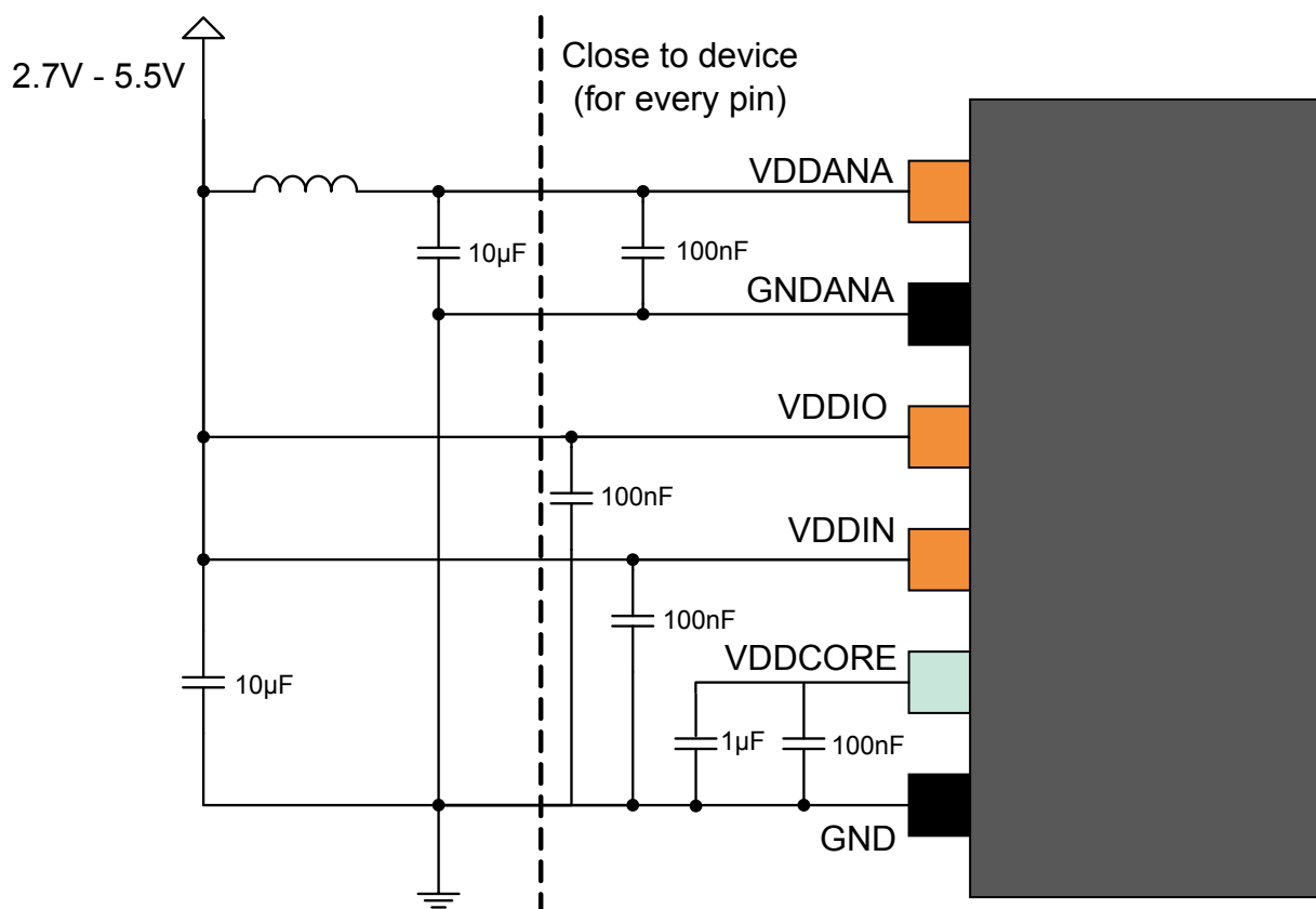
Figure 48-1. Single Power Supply Schematic
