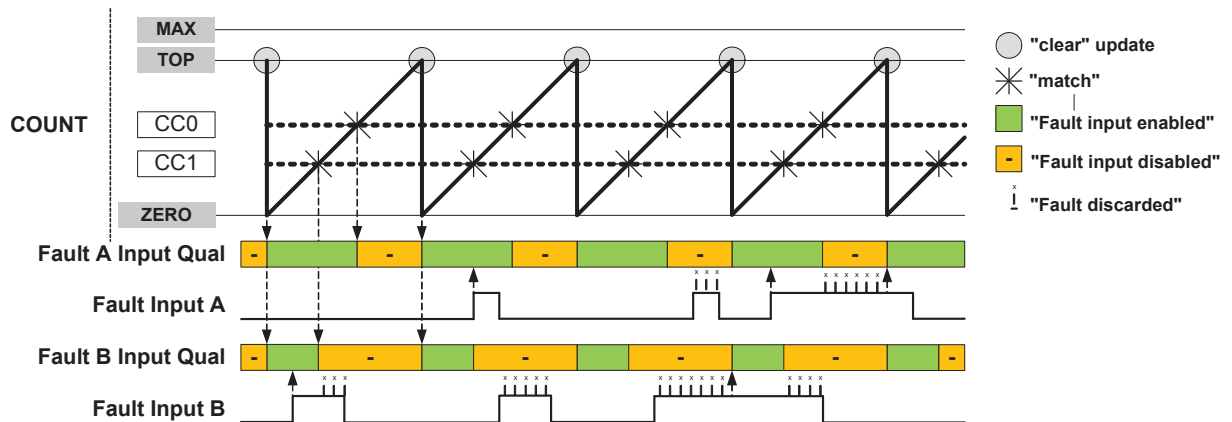
Figure 37-22. Fault Qualification in RAMP2 Operation with Inverted Polarity
