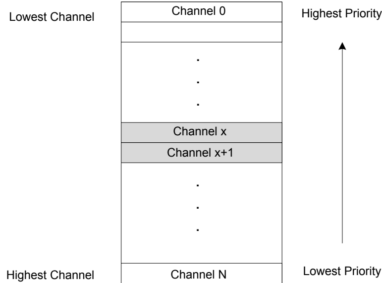
Figure 26-5. Static Priority Scheduling
