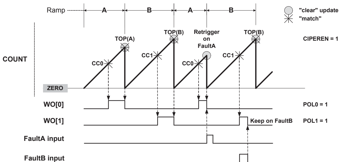
Figure 37-18. RAMP2 Standard Operation
