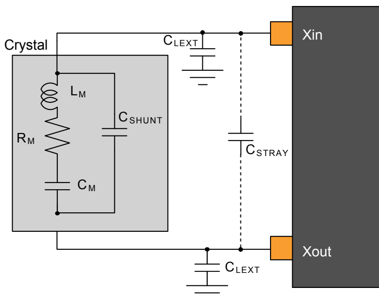
Figure 46-4. Oscillator Connection
