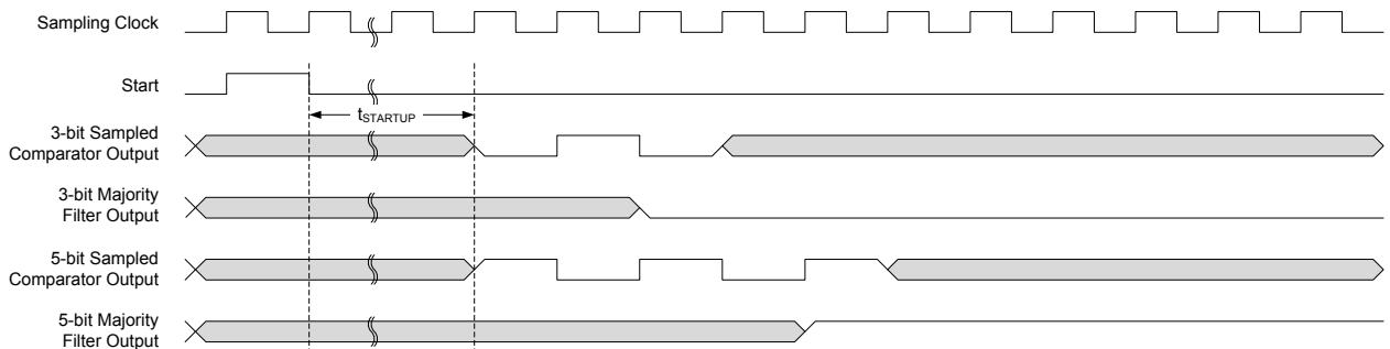
Figure 41-8. Single-Shot Filtering
