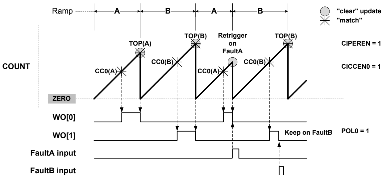
Figure 37-19. RAMP2 Alternate Operation
