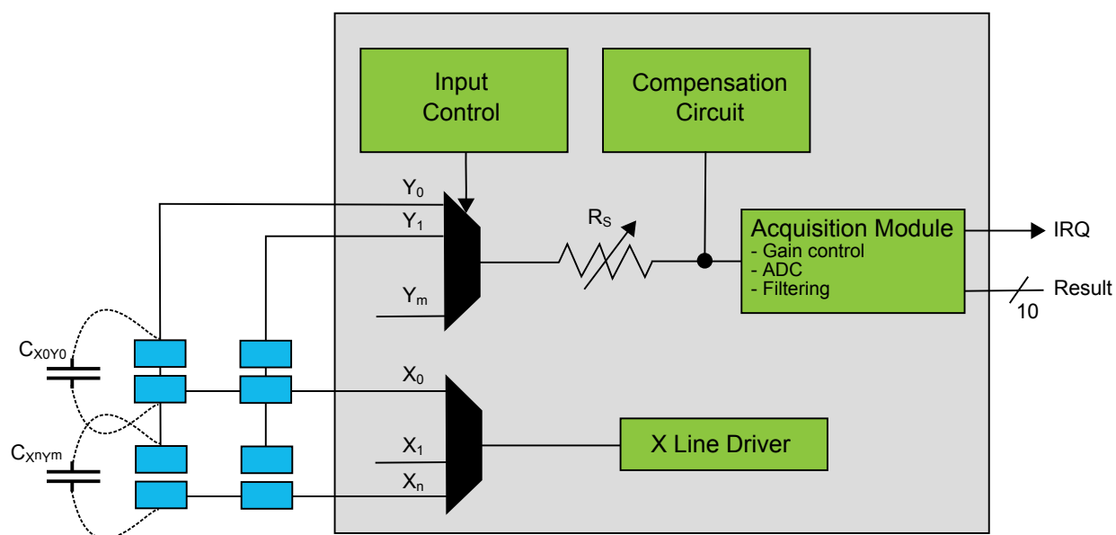
Figure 43-1. PTC Block Diagram Mutual-Capacitance
