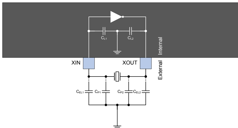
Figure 48-10. Crystal Circuit With Internal, External and Parasitic Capacitance
