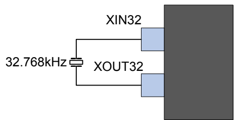
Figure 48-8. External Real Time Oscillator without Load Capacitor
