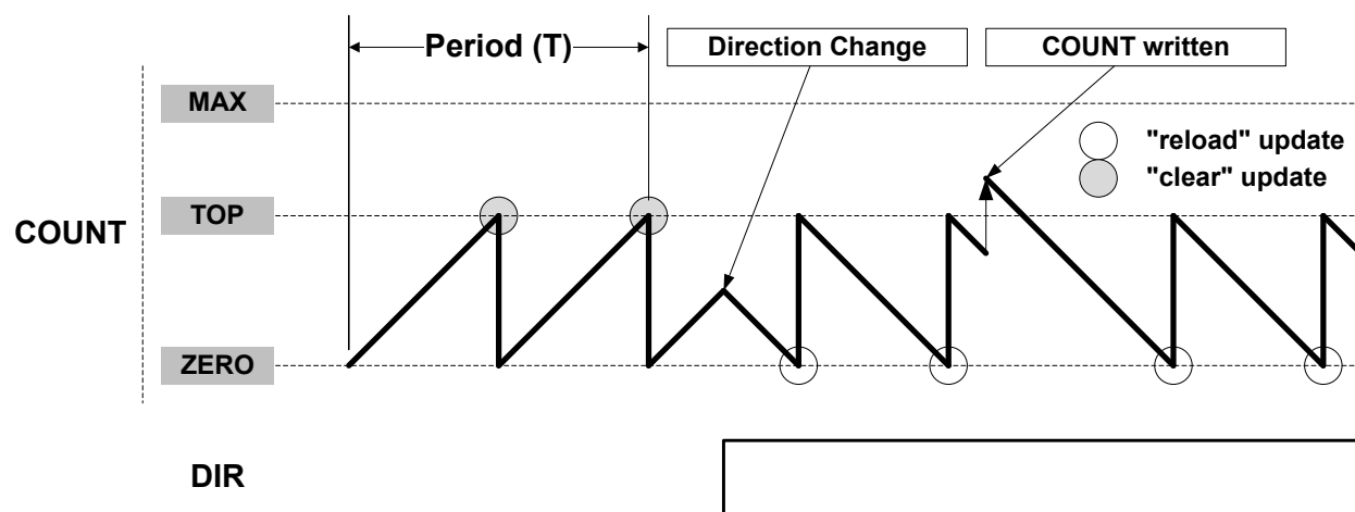
Figure 36-3. Counter Operation
