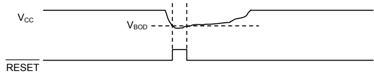
Figure 46-2. BODVDD Hysteresis OFF
