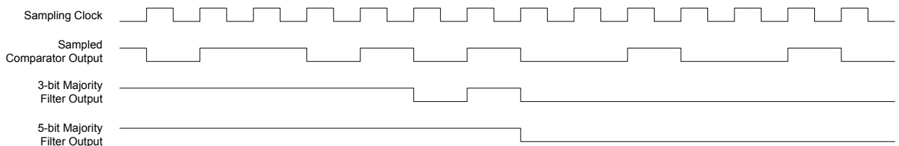
Figure 41-8. Single-Shot Filtering
