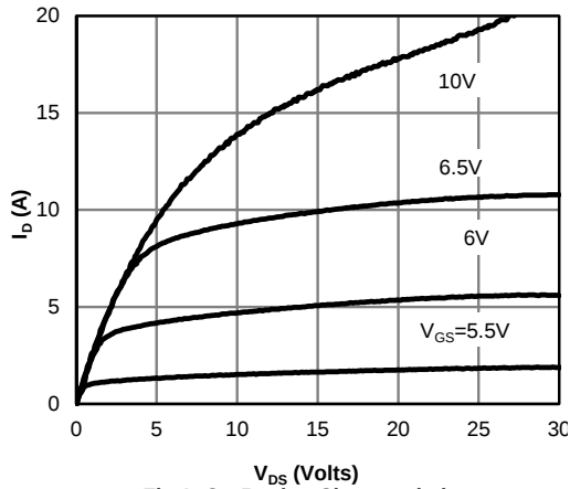
Fig 1: On-Region Characteristics
