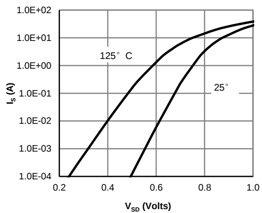
Figure 6: Body-Diode Characteristics
