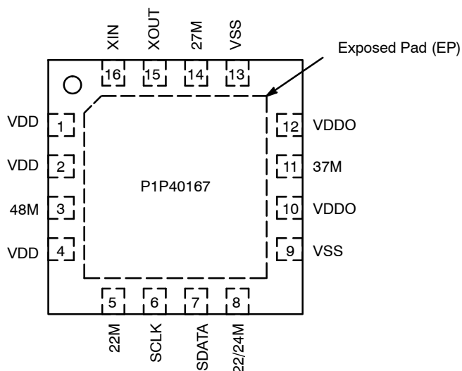
Figure 2. Pin Configuration (Top View)
