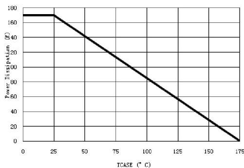
Figure 11: Power De-rating
