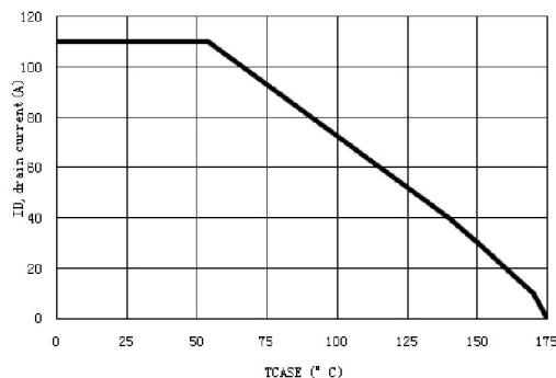
Figure 12: Current De-rating
