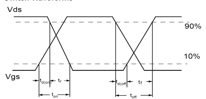
Switch Waveforms
