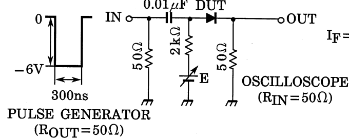
Fig.1 Reverse Recovery Time ( t_{rr} )
