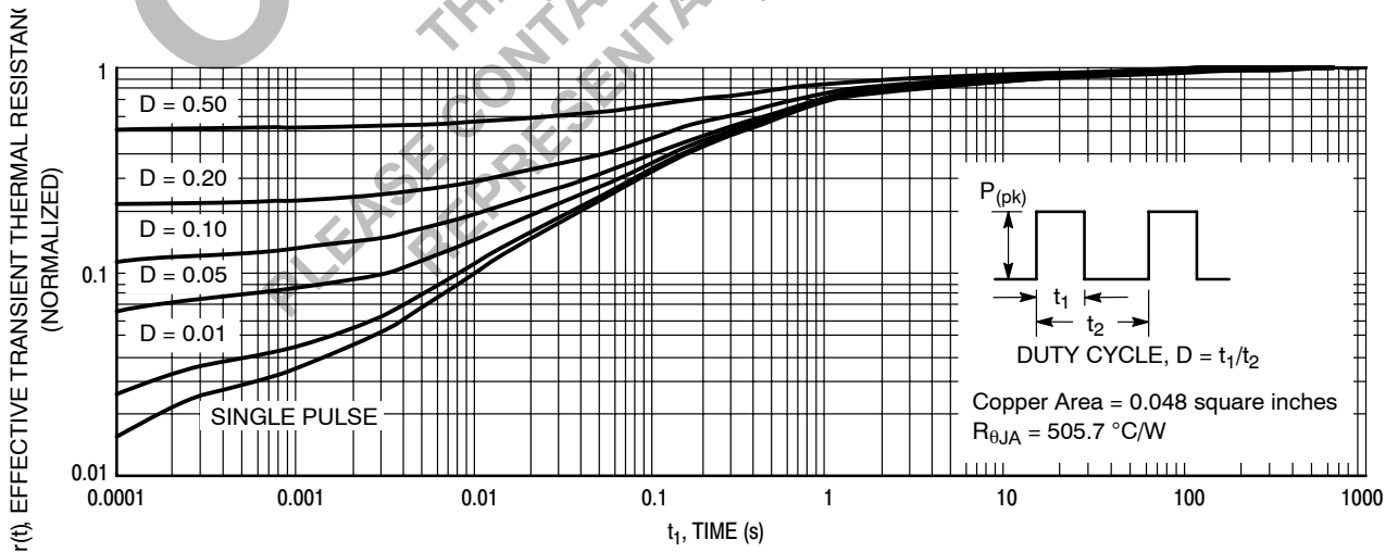
Figure 10. Normalized Thermal Response
