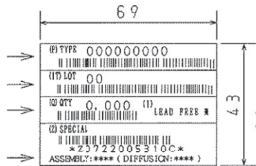
Reel label, Inner box label (unit :mm)
