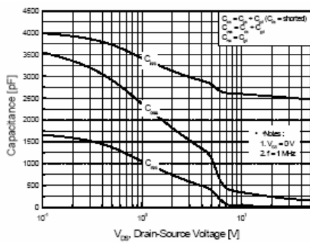
Figure 5. Capacitance Characteristics
