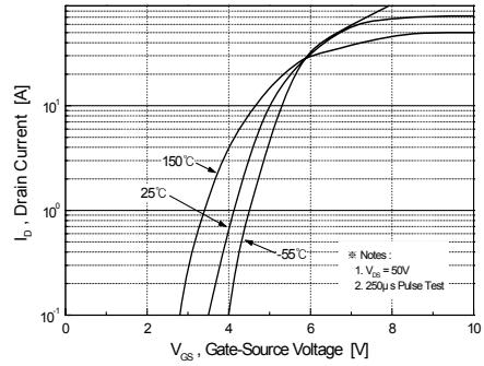
Figure 2. Transfer Characteristics
