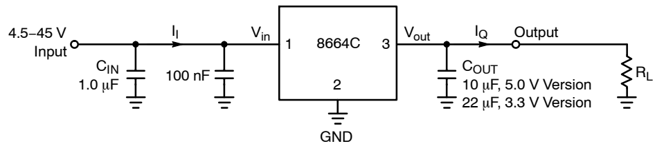
Figure 2. Measurement Circuit
