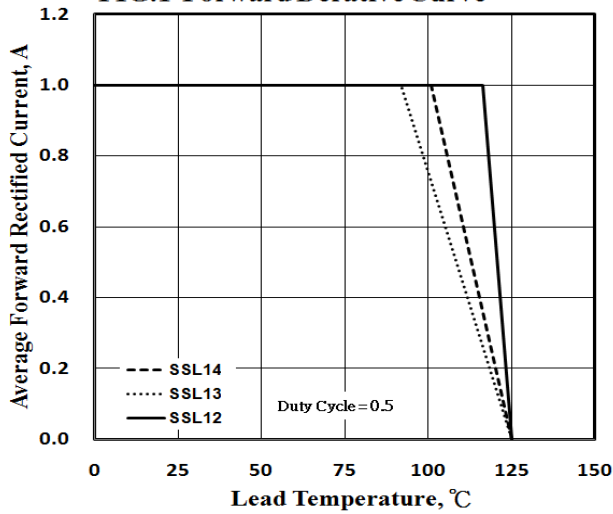
FIG.1-Forward Derivative Curve
