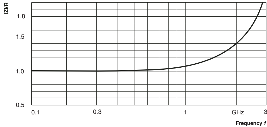
|Z|/R for 49.9 Ω MELF resistors
