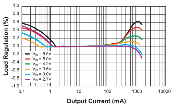
Load Regulation ( V_{OUT} = 1.2V ; L = 0.47\mu H )
