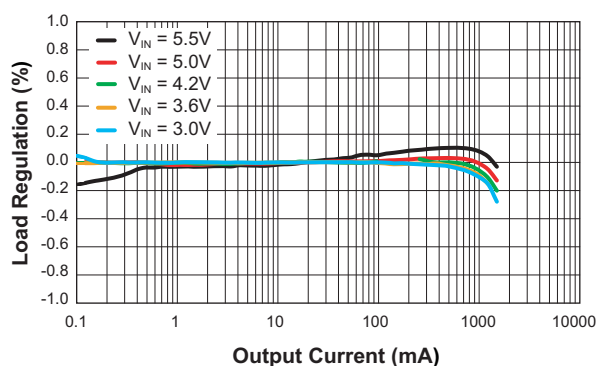
Load Regulation ( V_{OUT} = 2.5V ; L = 1\mu H )
