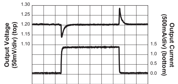
Load Transient
