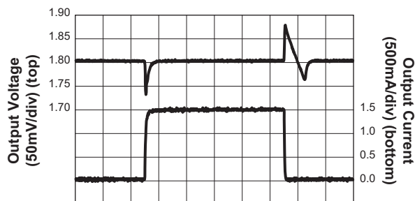
Load Transient
