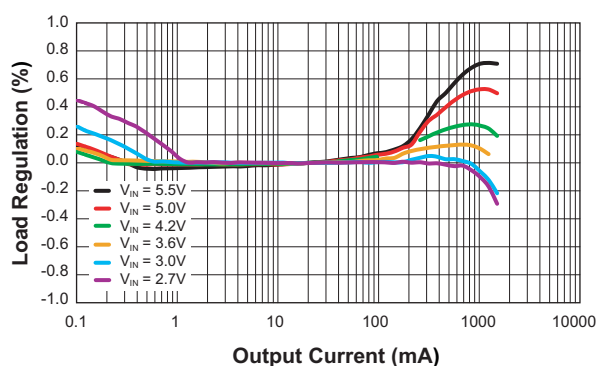
Load Regulation ( V_{OUT} = 1.8V ; L = 0.82\mu H )
