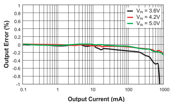
Load Regulation ( V_{OUT} = 3.3V ; L = 6.8\mu H ; C_{OUT} = 4.7\mu F )
