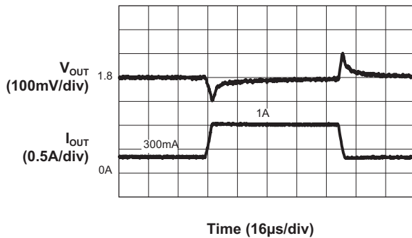
Load Transient
