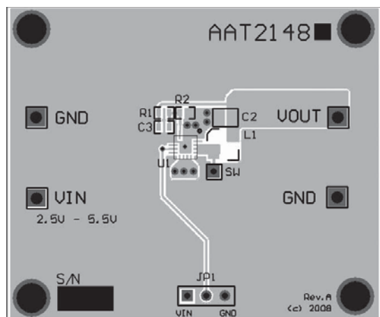
Figure 2: AAT2148 Evaluation Board Top Layer.
