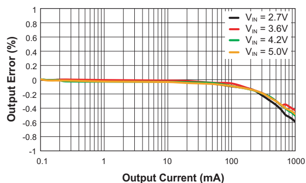
Load Regulation ( V_{OUT} = 1.2V ; L = 2.2\mu H ; C_{OUT} = 10\mu F )
