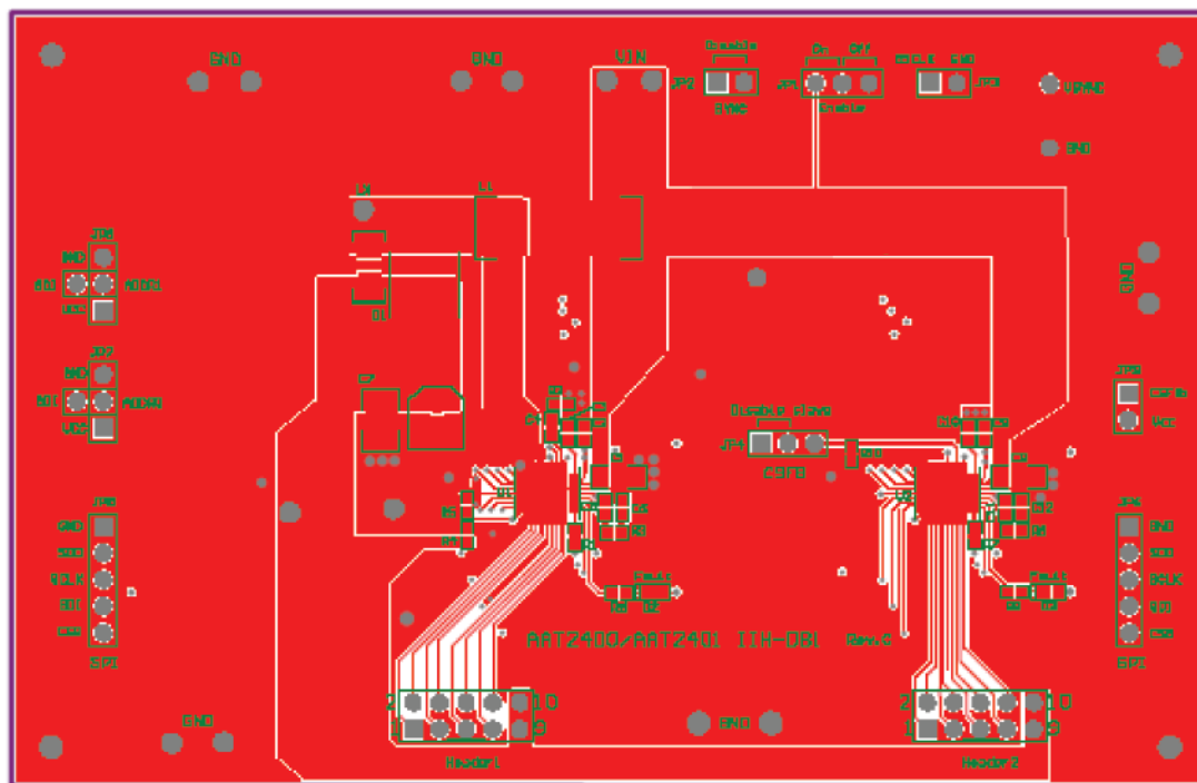
Figure 4: AAT2400 and AAT2401 Evaluation Board Top Side Layout.
