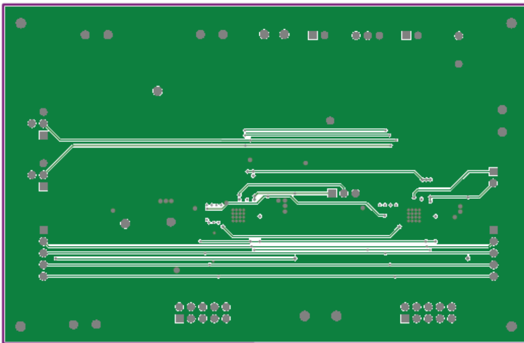
Figure 6: AAT2400 and AAT2401 Evaluation Board Middle-2 Layer Layout.
