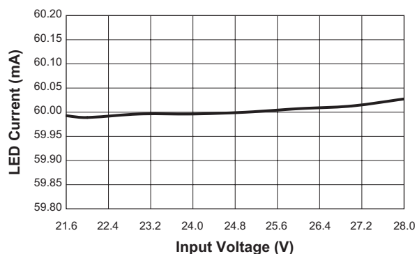
LED Current vs. Input Voltage (60mA/ch)
