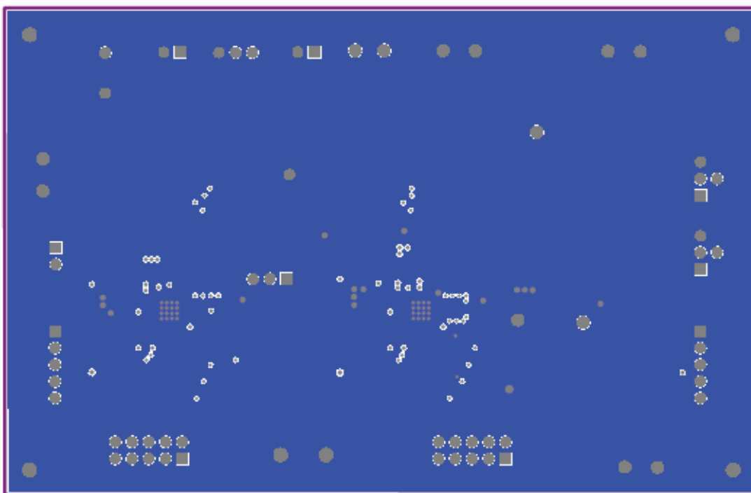
Figure 7: AAT2400 and AAT2401 Evaluation Board Bottom Side Layout.
