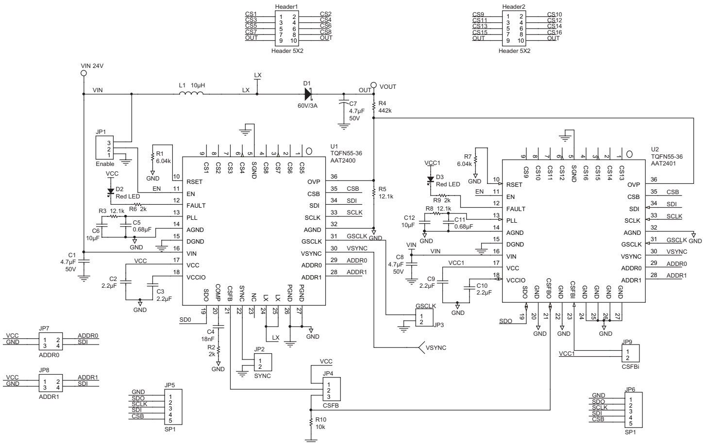
Figure 3: AAT2400 and AAT2401 DB1 Evaluation Board Schematic.
