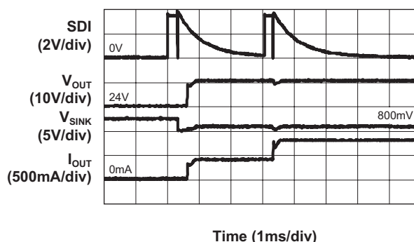
Turn On ( V_{IN} = 24V ; 50mA/ch)
