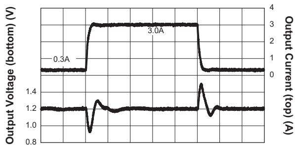
Step-Down Converter Load Transient Response ( I_{OUT} = 0.3A to 3.0A ; V_{IN} = 3.6V ; V_{OUT} = 1.2V ; C_{OUT} = 22\mu F )
