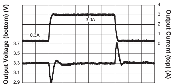
Step-Down Converter Load Transient Response ( I_{OUT} = 0.3A to 3.0A ; V_{IN} = 4.2V ; V_{OUT} = 3.3V ; C_{OUT} = 22\mu F )
