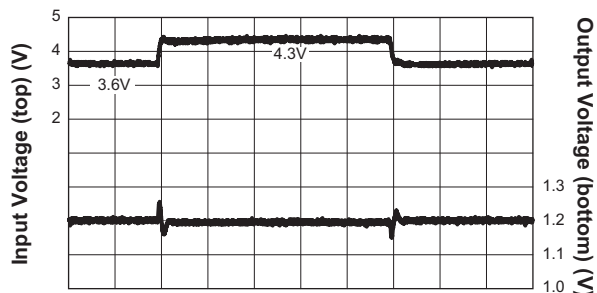
Step-Down Converter Line Transient Response ( V_{IN} = 3.6V to 4.3V ; V_{OUT} = 1.2V ; I_{OUT} = 3A )
