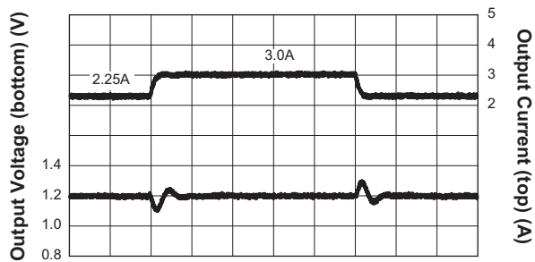
Step-Down Converter Load Transient Response ( I_{OUT} = 2.25A to 3.0A ; V_{IN} = 3.6V ; V_{OUT} = 1.2V ; C_{OUT} = 22\mu F )
