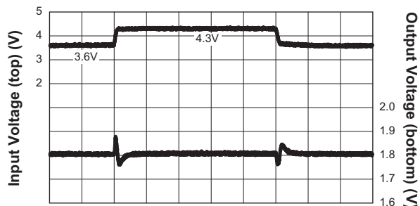
Step-Down Converter Line Transient Response ( V_{IN} = 3.6V to 4.3V ; V_{OUT} = 1.8V ; I_{OUT} = 3A )
