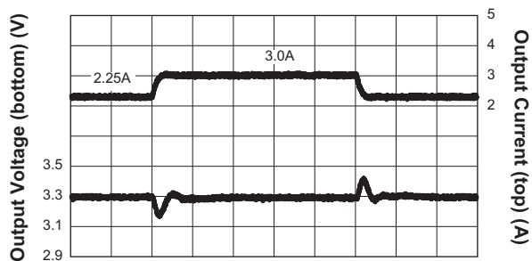
Step-Down Converter Load Transient Response ( I_{OUT} = 2.25A to 3.0A ; V_{IN} = 4.2V ; V_{OUT} = 3.3V ; C_{OUT} = 22\mu F )
