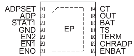
AAT3672-3
