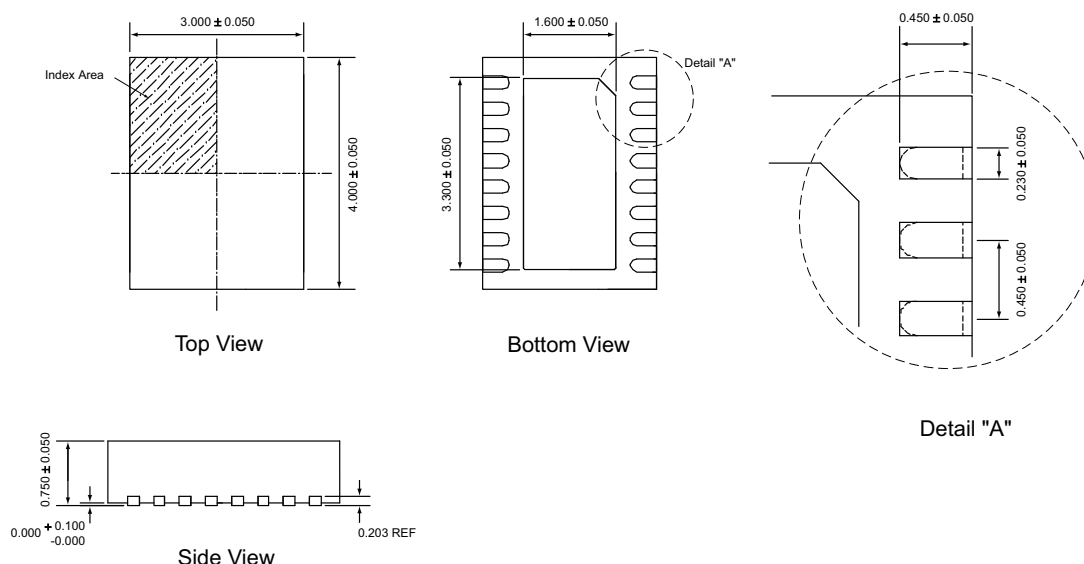
TDFN34-16 3
