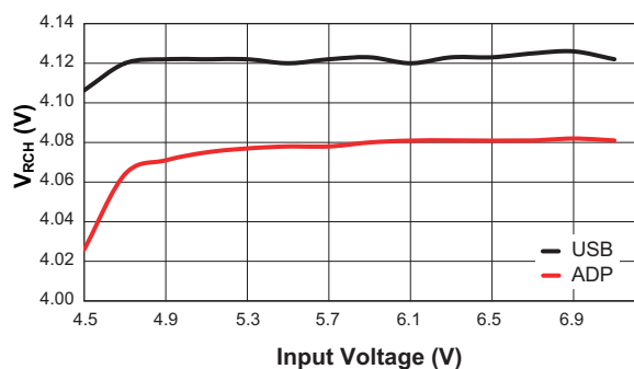
Battery Recharge Voltage Threshold vs. Input Voltage ( R_{ADPSET} = 1k\Omega ; R_{USBSET} = 3.2k\Omega ; C_{BAT} = 22\mu F )
