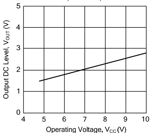
Output DC Level vs. Operating Voltage ( T_a = 25^\circ\text{C} )
