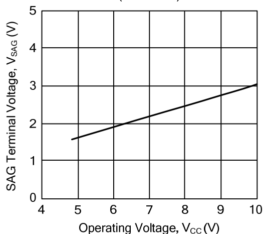
SAG Terminal Voltage vs. Operating Voltage ( T_a = 25^\circ\text{C} )
