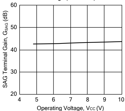
SAG Terminal Gain vs. Operating Voltage ( T_a = 25^\circ\text{C} )
