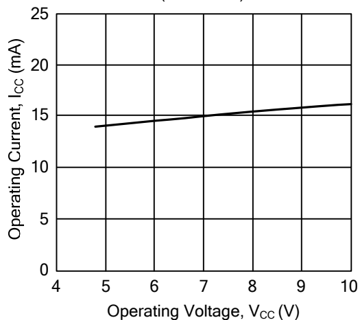
Operating Current vs. Operating Voltage ( T_a = 25^\circ\text{C} )
