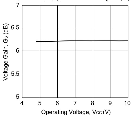
Voltage Gain vs. Operating Voltage ( T_a = 25^\circ\text{C} , 1Vp-p, 1MHz sinewave signal input)
