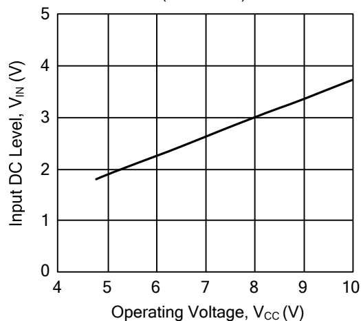
Input DC Level vs. Operating Voltage ( T_a = 25^\circ\text{C} )
