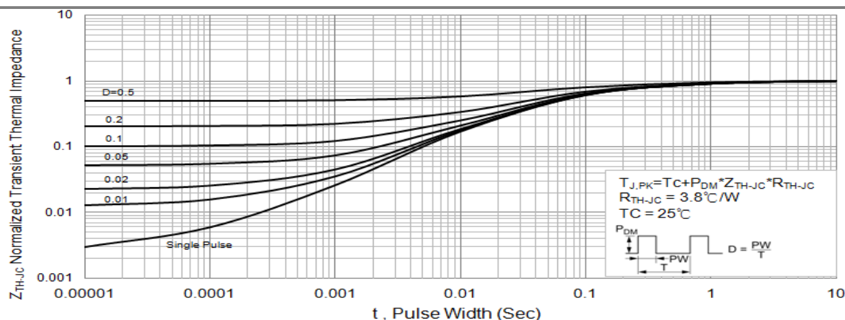
Fig.15 PJF4NA70 Normalized Transient Thermal Impedance vs. Pulse Width
