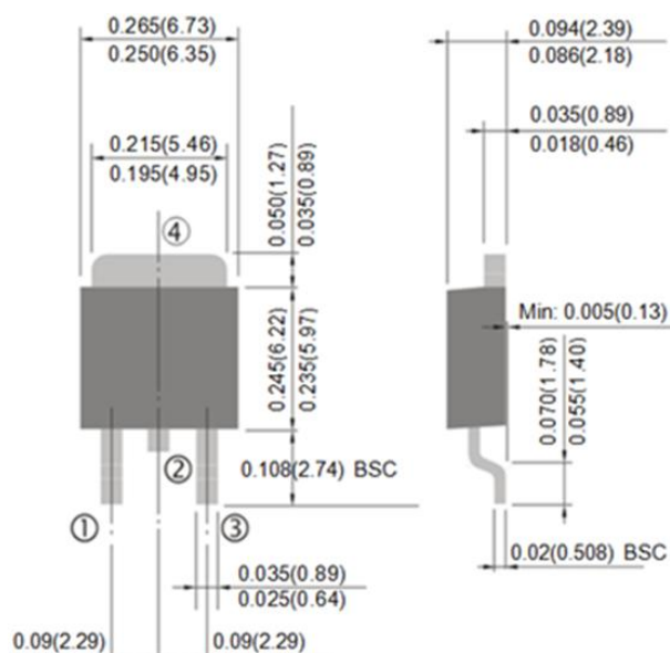
TO-252AA Dimension
