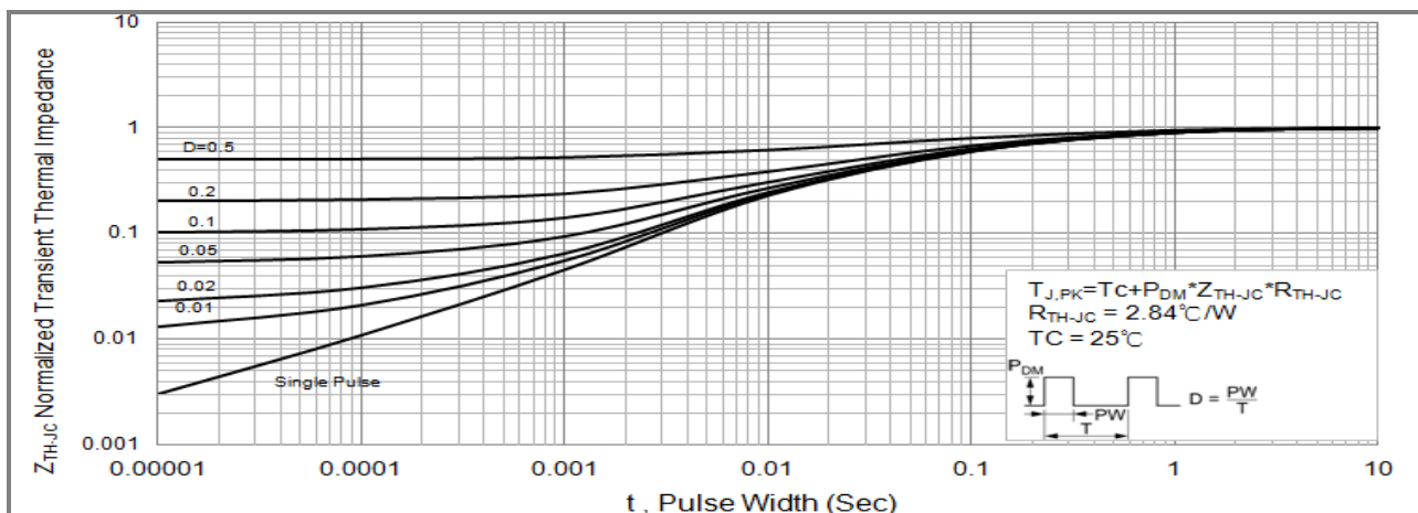
Fig.15 PJF4NA90 Normalized Transient Thermal Impedance vs. Pulse Width
