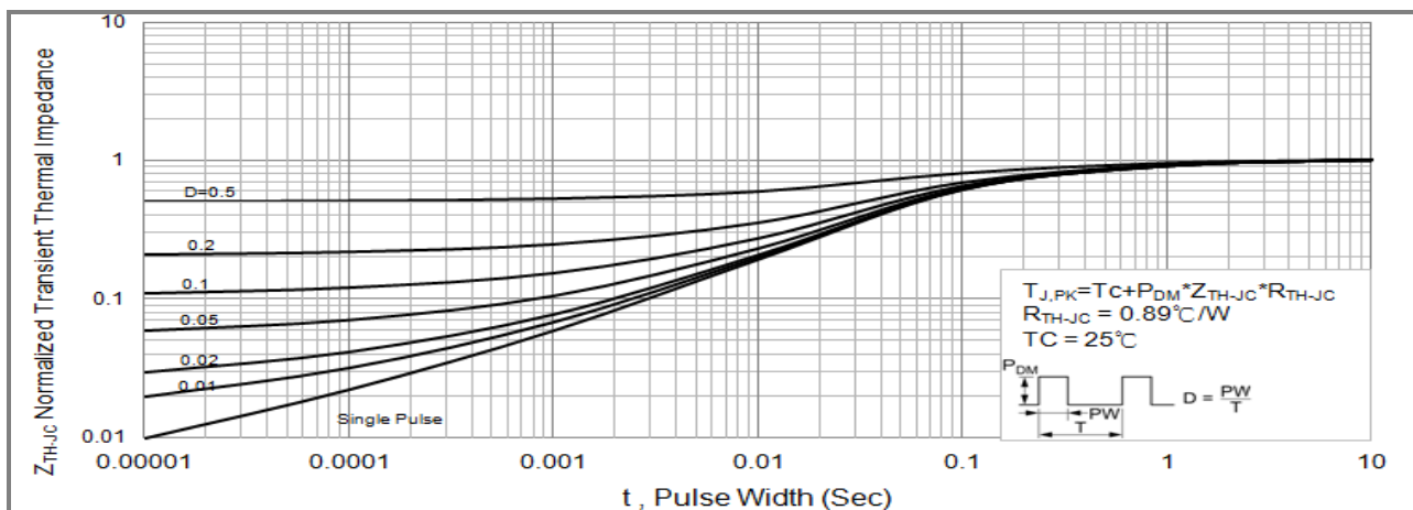
Fig.14 PJP4NA90 Normalized Transient Thermal Impedance vs. Pulse Width
