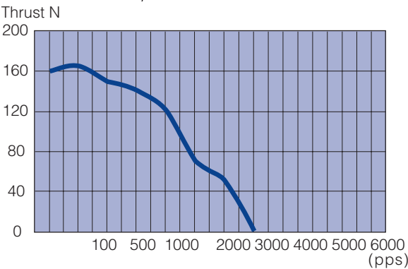
Speed Vs Thrust 11HS1002-14 0.7A/24V
