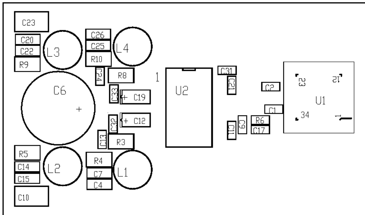
Figure 6. Silkscreen Layer
