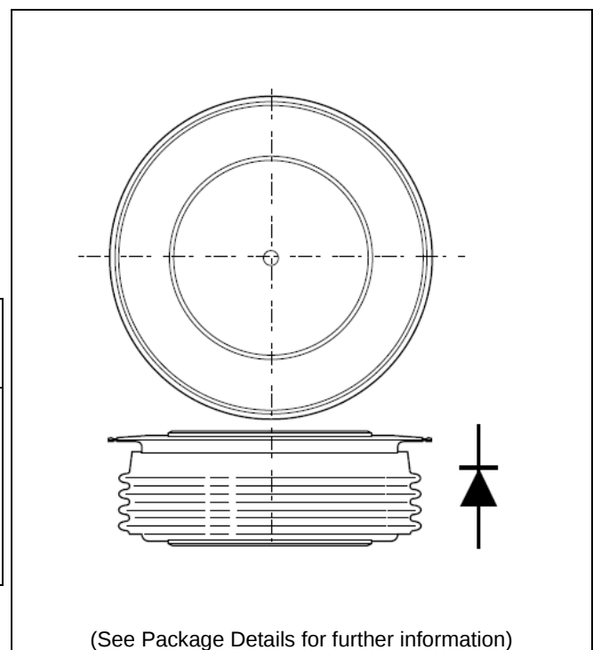
Fig. 1 Package outline
