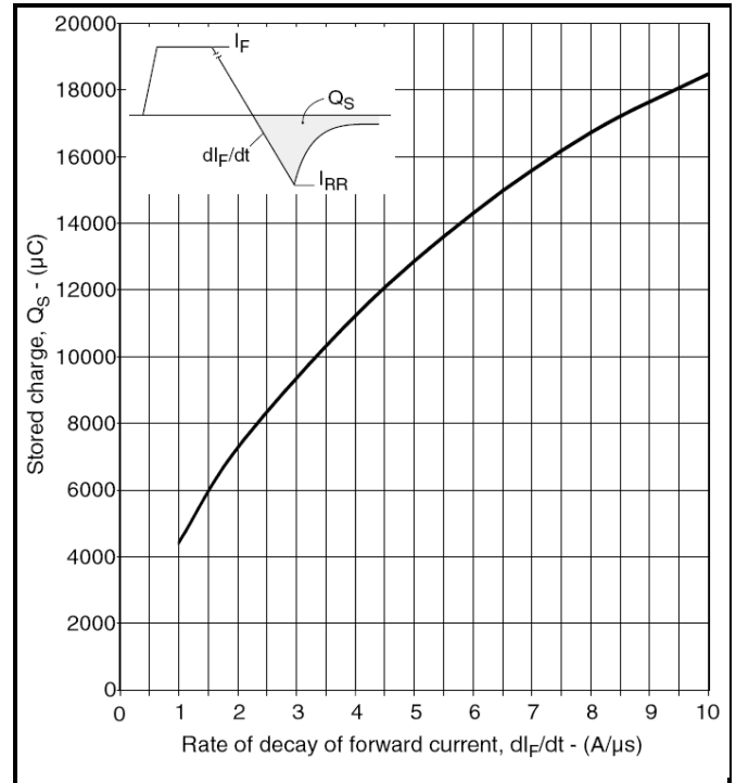
Fig.5 Stored charge
