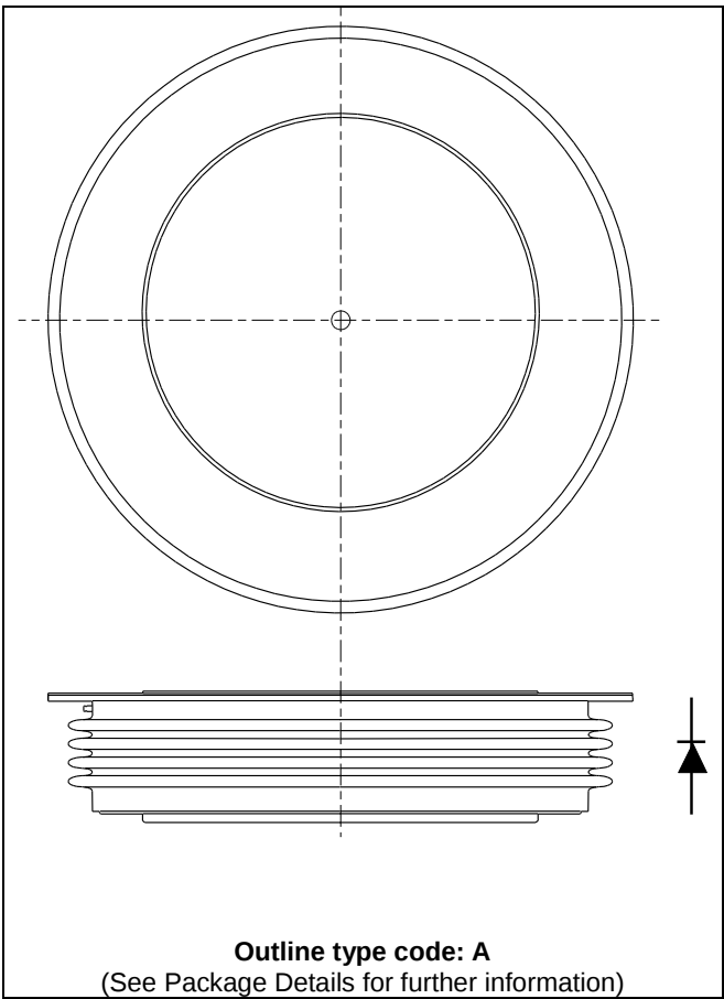
Fig. 1 Package outlines
