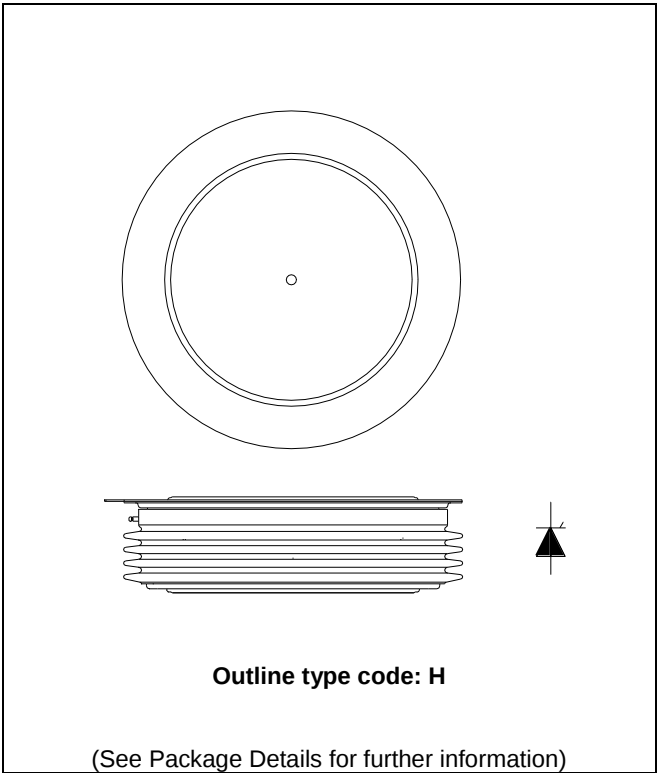
Fig. 1 Package outline
