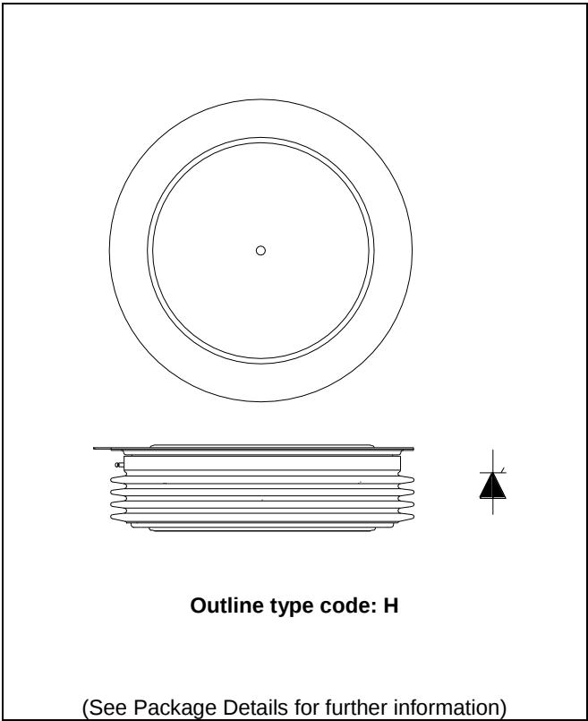
Fig. 1 Package outline
